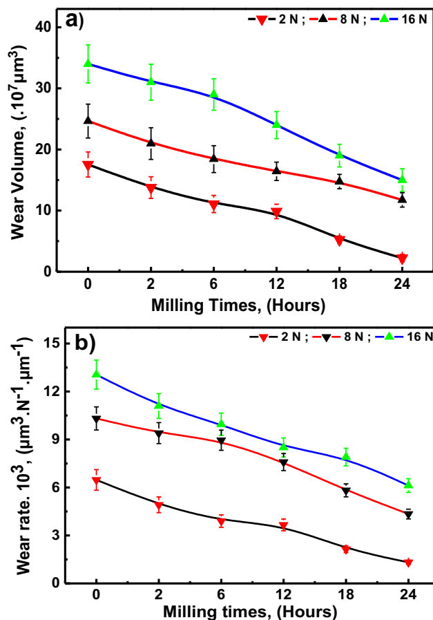
Fig. 12 Development of: (a) wear capacity (μm 3 ), and (b) wear rate (μm 3 ·N -1 ·μm -1 ) of milled Al 2 O 3 -α as a function of milling times (h) at diverse applied load (N).
