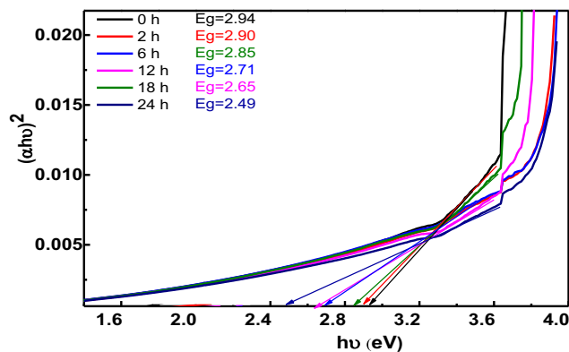
Fig. 16 Tauc plot of Milled \alpha - \text{Al}_2\text{O}_3 with different milling times for determining the band gap.
