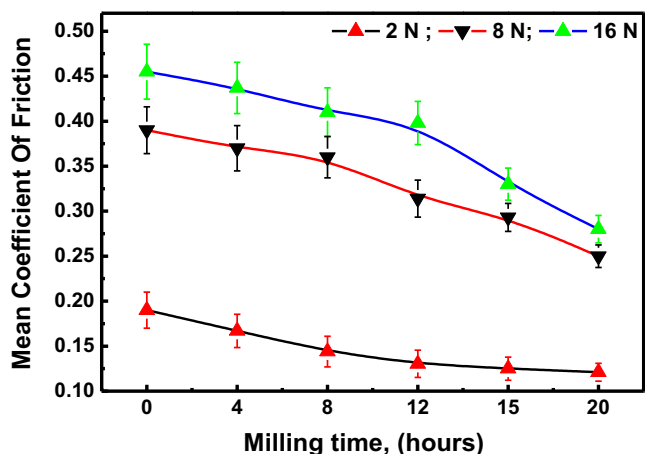
Fig. 11 Mean friction coefficients of milled Al 2 O 3 -α as a function of milling times (h), under different applied load (N).
