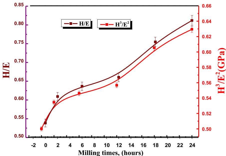
Fig. 10 H/E and H 3 /E 2 ratio's of α-Al 2 O 3 samples as a function of milling times.
