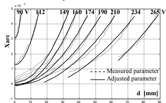
a. Variation of X_{arc}
