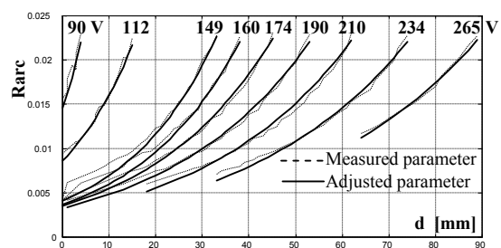
b. Variation of R_{arc}
