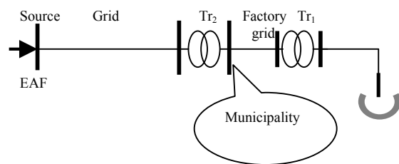
a. EAF supply.
