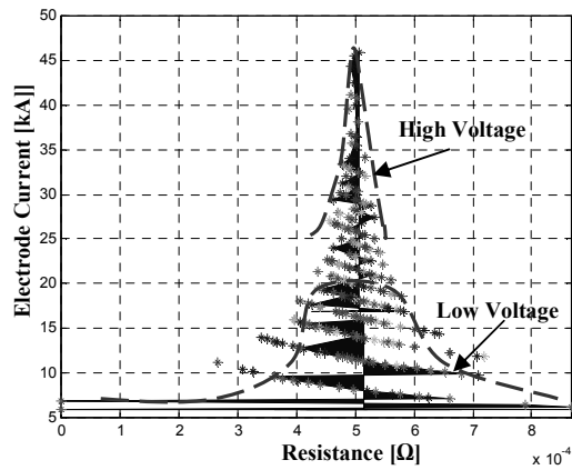
a. Distribution of R_1
